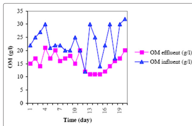
Figure 5: Organic matters before and after treatment in digester
