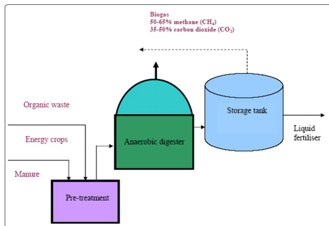
Figure 1: General schematic of an agricultural biogas plant [6].
