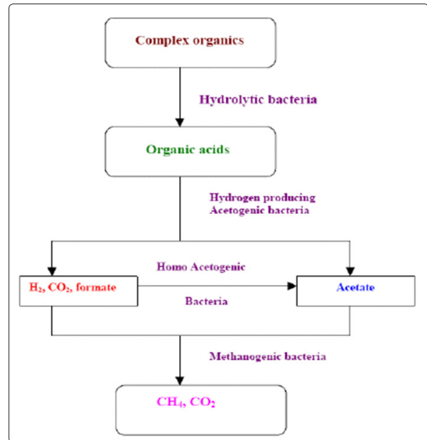
Figure 3: Biogas production processes [6].
