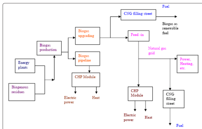
Figure 4: Overview of biogas utilisation pathways [13].
